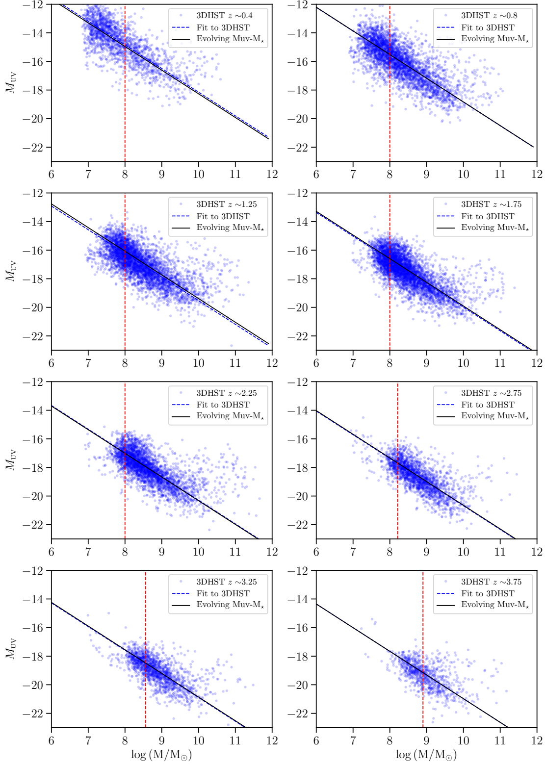
Figure 6. The M_{UV}-M_{*} relation for realizations of the SED-fitting of observed star-forming galaxies ( \log(\text{sSFR}) < -10 \text{ Gyr}^{-1} ) in the 3DHST survey (blue points) with high-confidence measurements of M_{UV} , M , and redshift as described in Sections 3.2 and 3.4.1. Blue dashed lines indicate the best-fitting linear relationship under the assumption of a fixed slope as described in the text. Solid black lines indicate the smoothly evolving redshift-evolution of the M_{UV}-M_{*} relation in our model as characterized in Figure 7 and Equation 11. The red dashed line indicates the stellar mass above which mock galaxies are matched to 3DHST realizations, which is the larger between \log(M/M_{\odot}) > 8 and \log(M/M_{\odot}) > 6.3 + 0.7z (the evolving mass limit exceeds \log(M/M_{\odot}) > 8 at z > 2.4 ).
